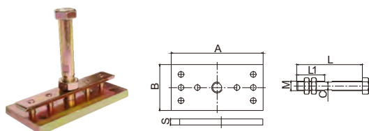
固定件 Adjustable Pin with Plate for Fastening
