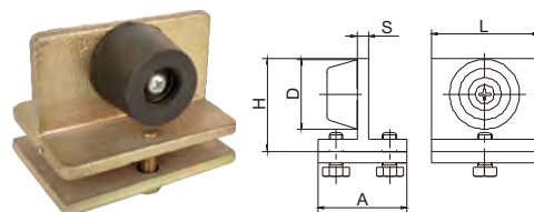
折叠门门吸 Sliding and Folding Door Stopper
