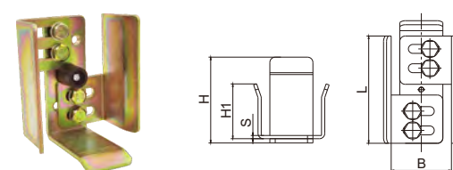
双向调节门兜 Adjustable Stopper for Sliding and Folding Door
