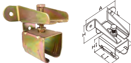
折叠门轨道托架 Wall Fixing Bracket Height Adjusted
