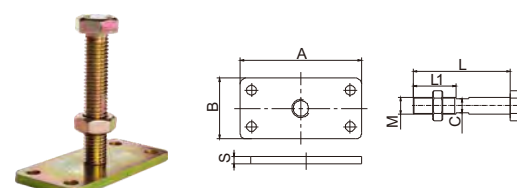
固定件 Adjustable Pin with Plate for Fastening
