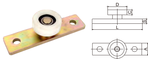
折叠门尼龙导轮 (带固定板) Nylon Guide Roller with Fixing Plate
